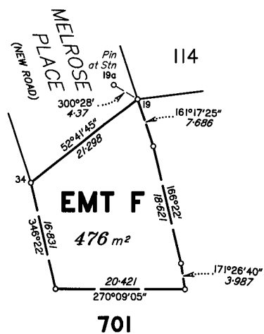
DIAGRAM B 1: 500
