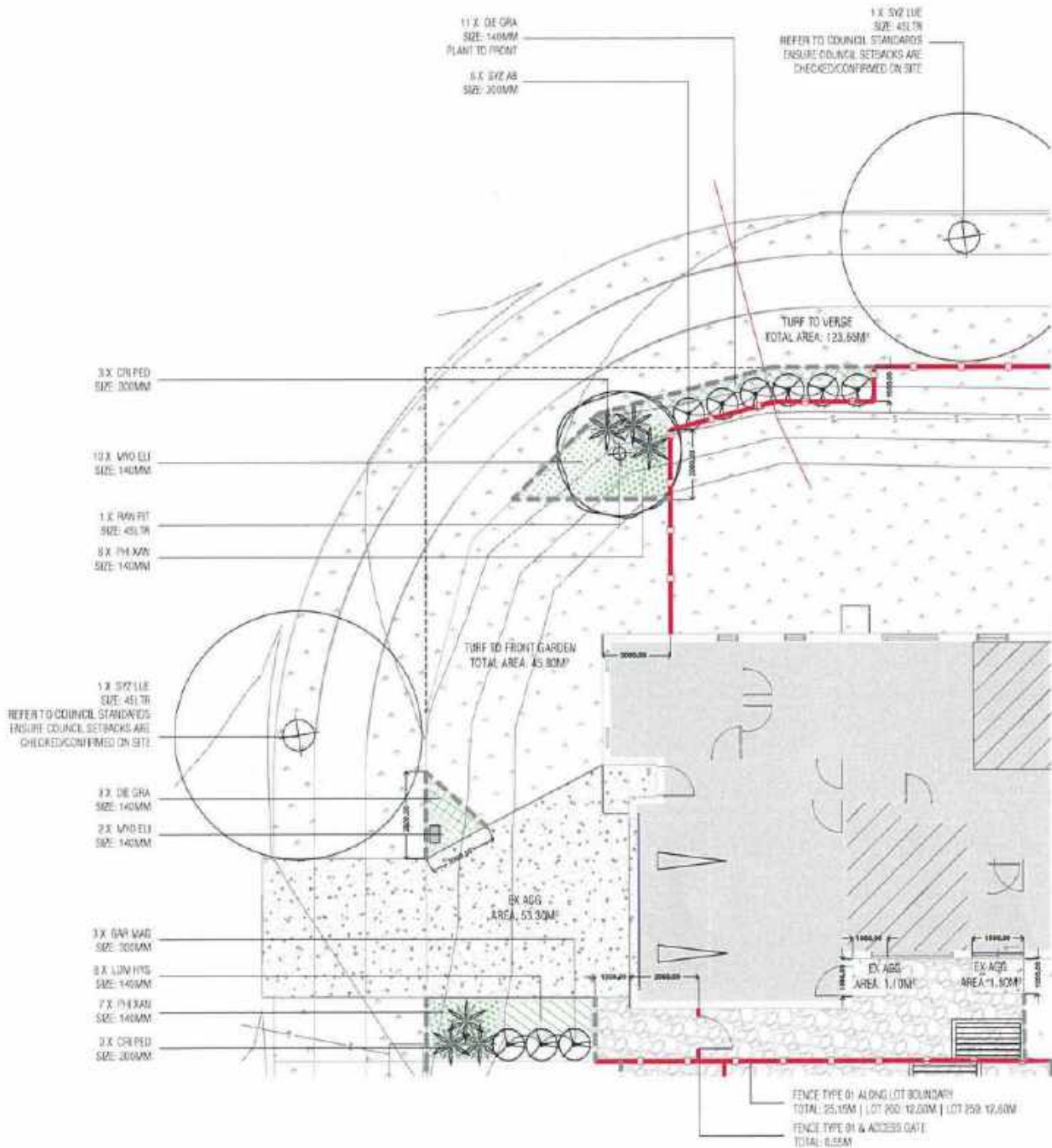
LANDSCAPE PLAN B: EXAMPLE LANDSCAPE PLAN FOR A CORNER BLOCK
