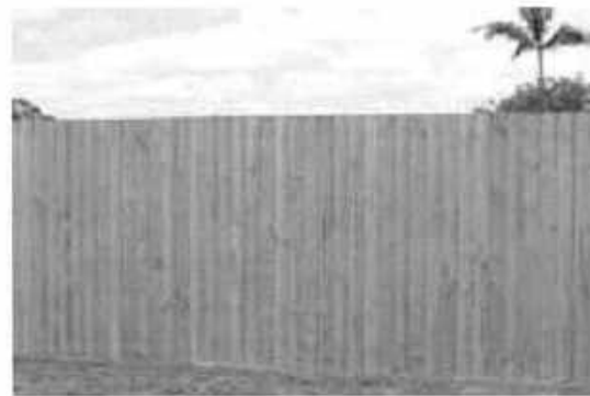
DIAGRAM D: PALING FENCING Fencing is to be timber, 1800mm high and 100% solid. Must be constructed of A grade CCA treated pine timber palings (3 rails, palings to front side and timber posts).
