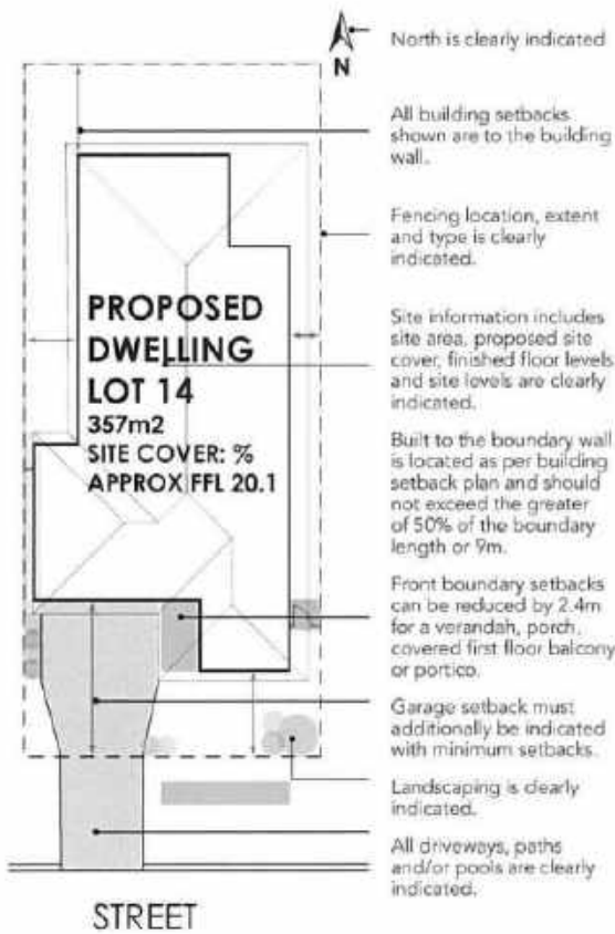
DIAGRAM A: EXAMPLE SITE PLAN FOR STANDARD BLOCK
